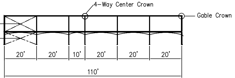
SIDE VIEW
