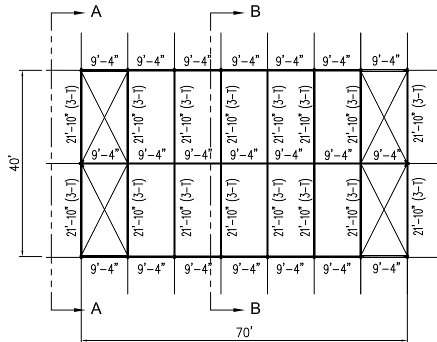
PLAN VIEW
