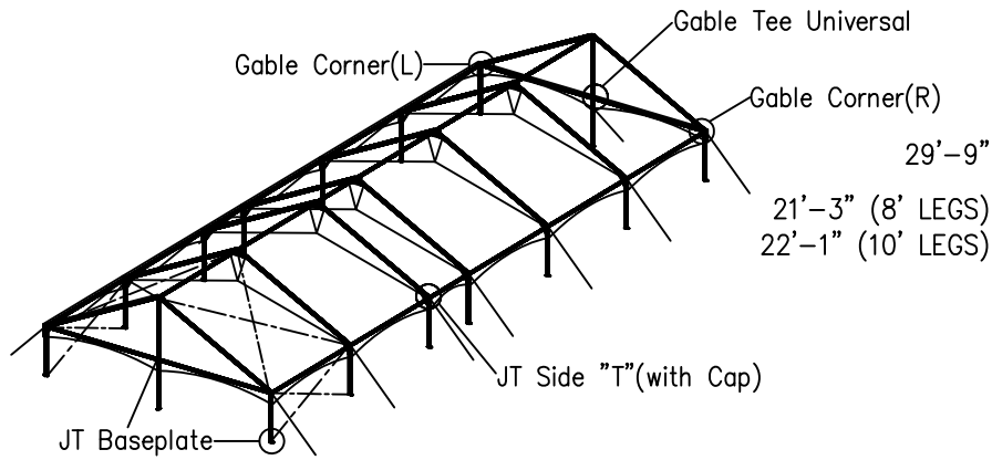
ISOMETRIC VIEW
