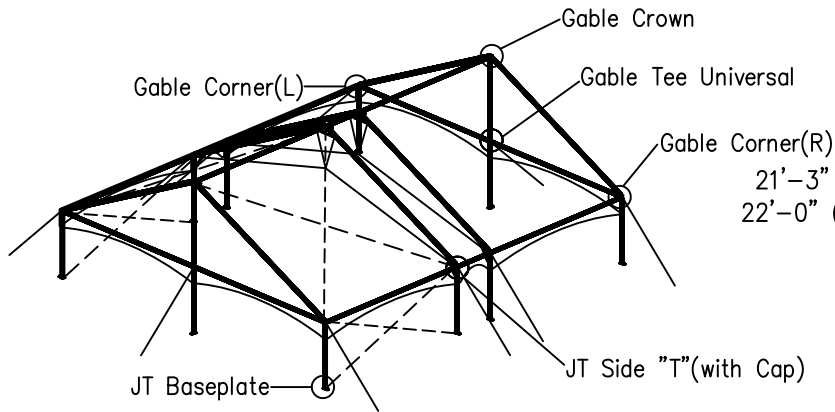
ISOMETRIC VIEW
