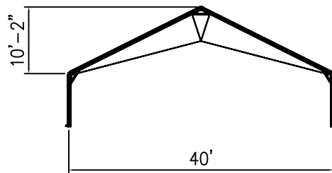
VIEW B-B
