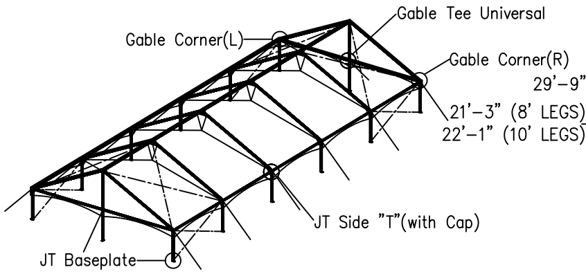
ISOMETRIC VIEW
