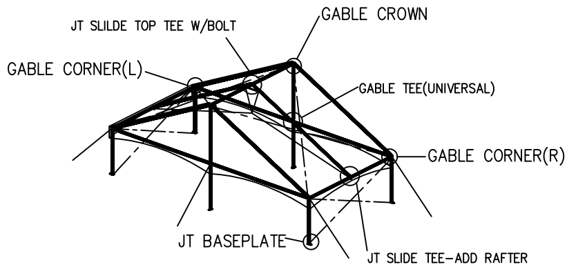
ISOMETRIC VIEW
