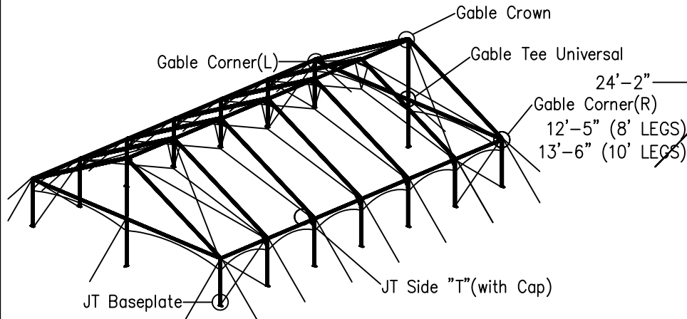
ISOMETRIC VIEW
