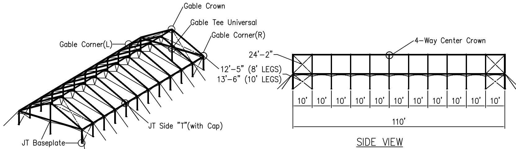
ISOMETRIC VIEW
