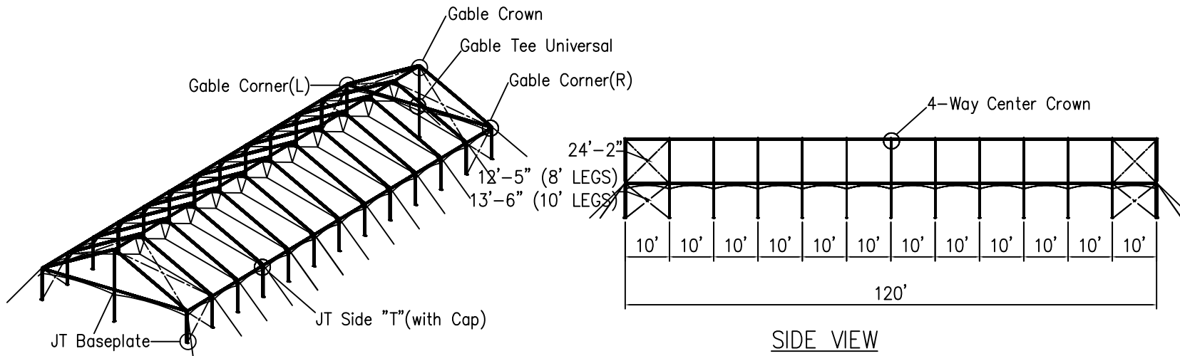
ISOMETRIC VIEW
