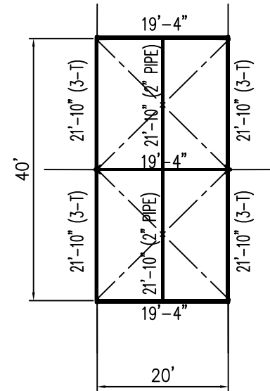
PLAN VIEW
