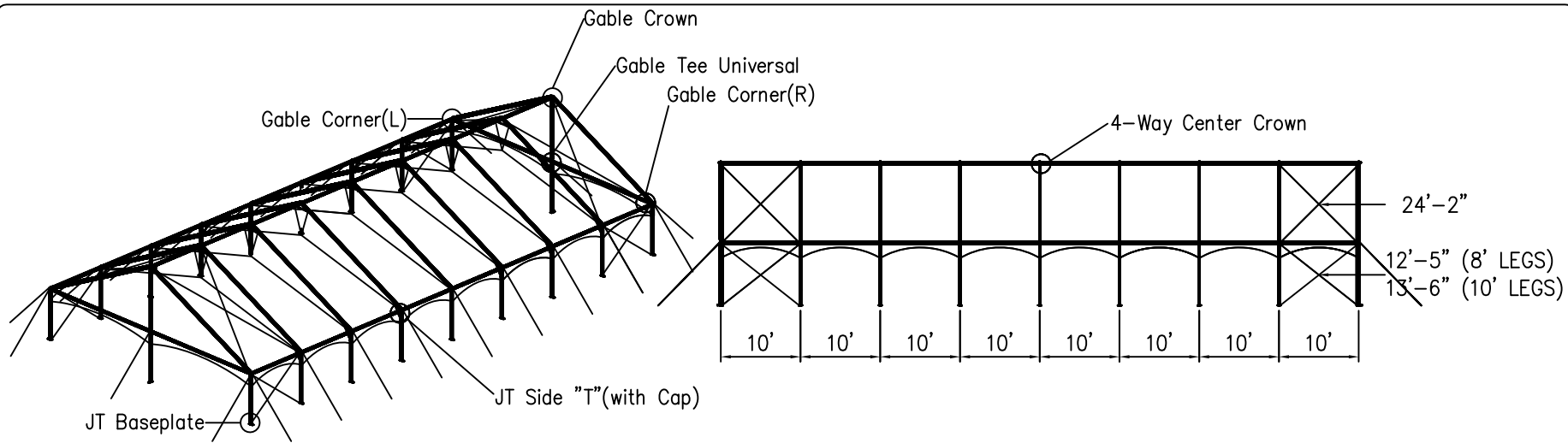
SIDE VIEW
