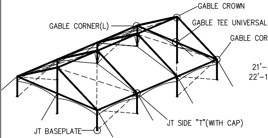
ISOMETRIC VIEW
