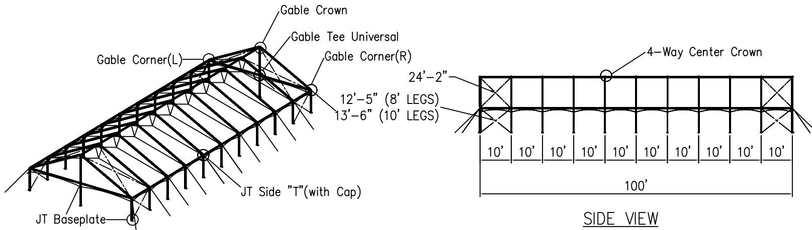
ISOMETRIC VIEW
