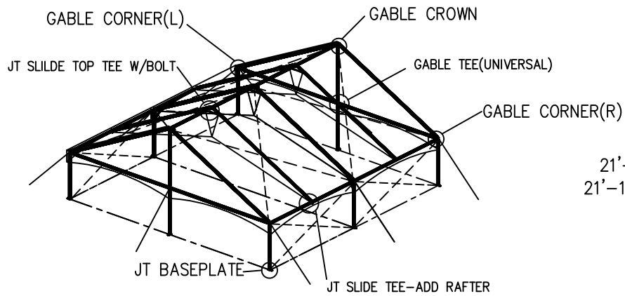
ISOMETRIC VIEW
