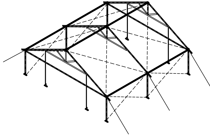
ISOMETRIC VIEW
