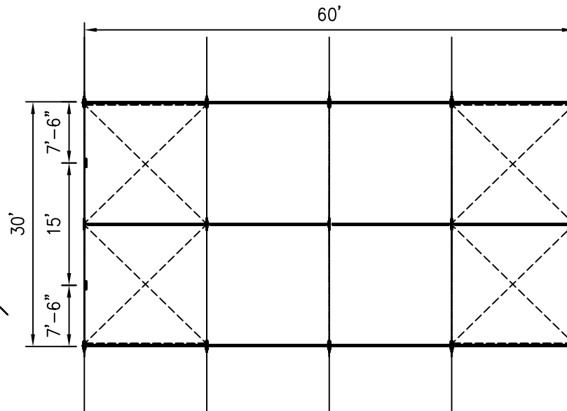
PLAN VIEW
