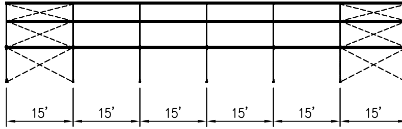
SIDE VIEW
