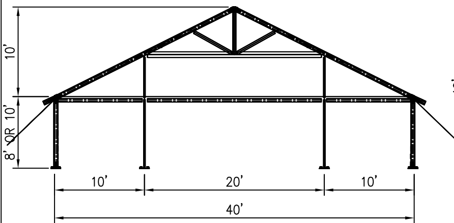
PLAN VIEW
