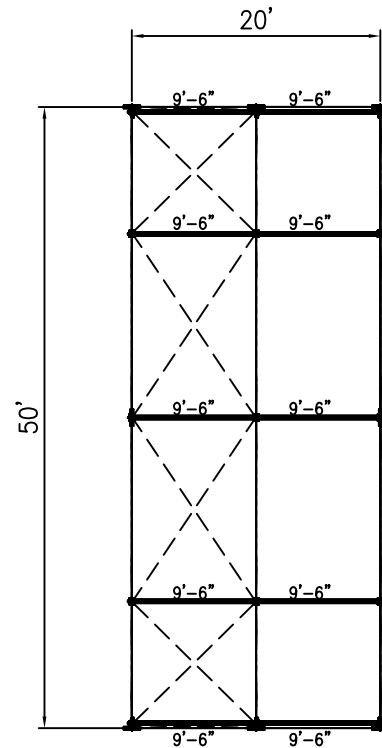
PLAN VIEW
