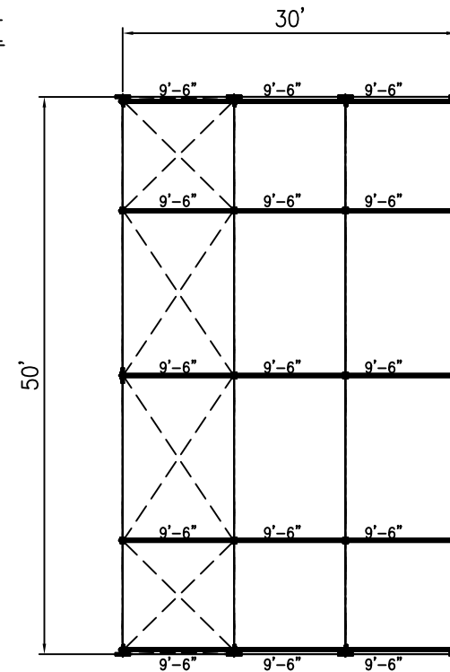
PLAN VIEW
