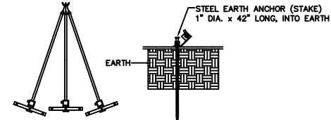
DETAIL OF STAKE BAR ASSEMBLY
