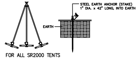
DETAIL OF STAKE BAR ASSEMBLY
