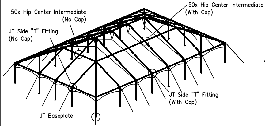
ISOMETRIC VIEW
