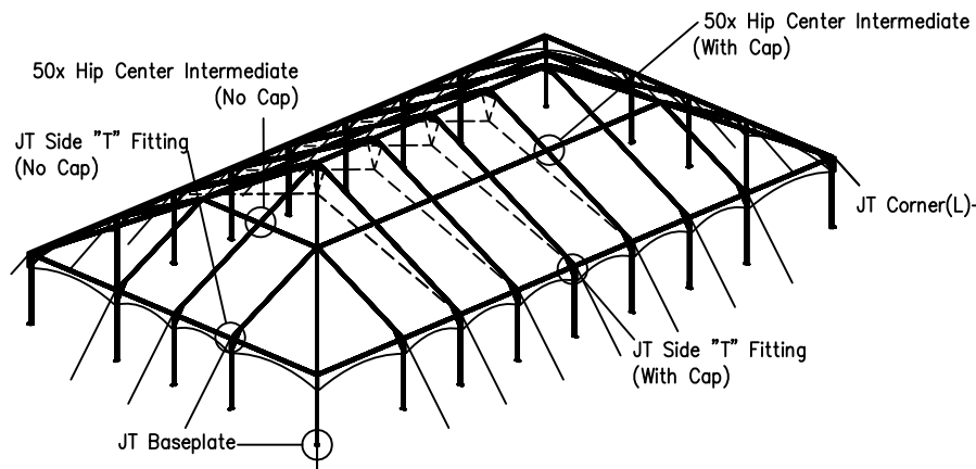
ISOMETRIC VIEW
