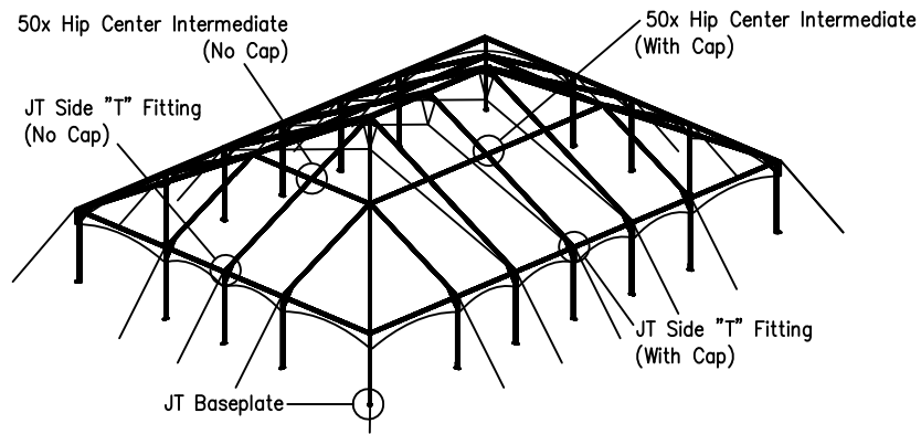
ISOMETRIC VIEW
