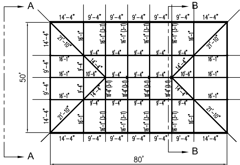
PLAN VIEW
