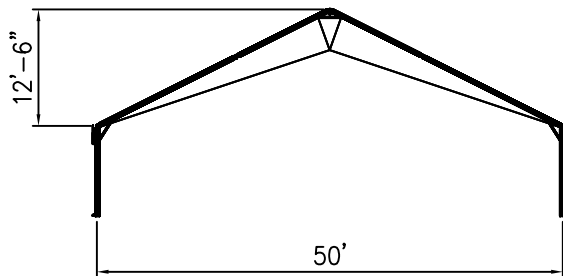
VIEW B-B
