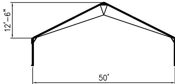
VIEW B-B
