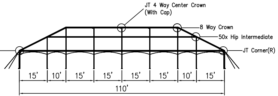
SIDE VIEW
