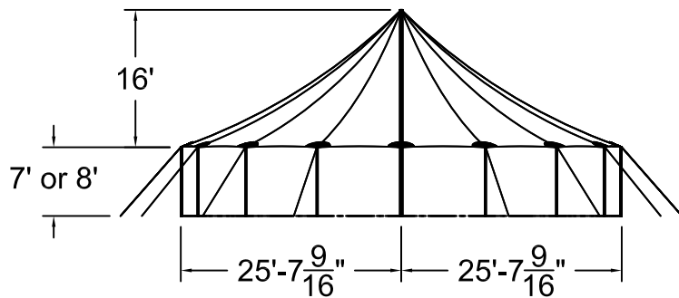
51'W TW FRONT END
