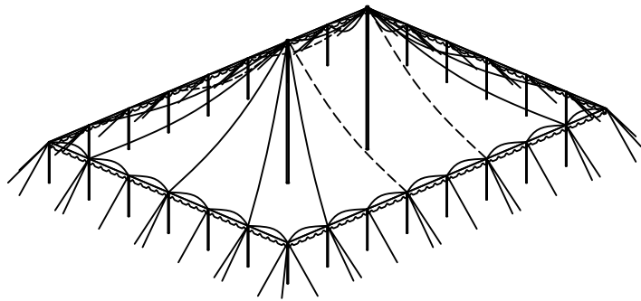
ISOMETRIC VIEW
