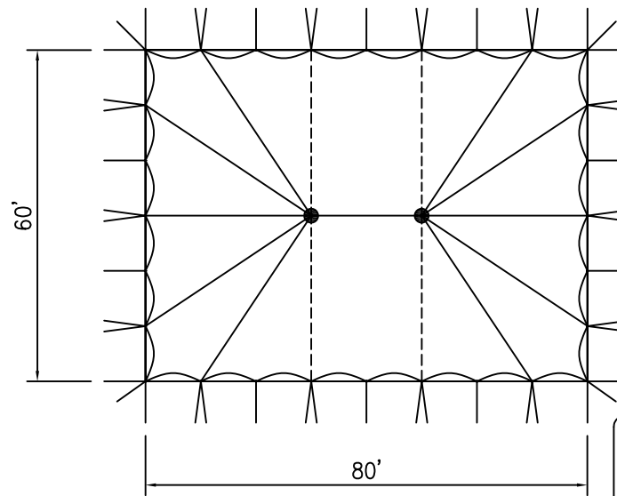
PLAN VIEW
