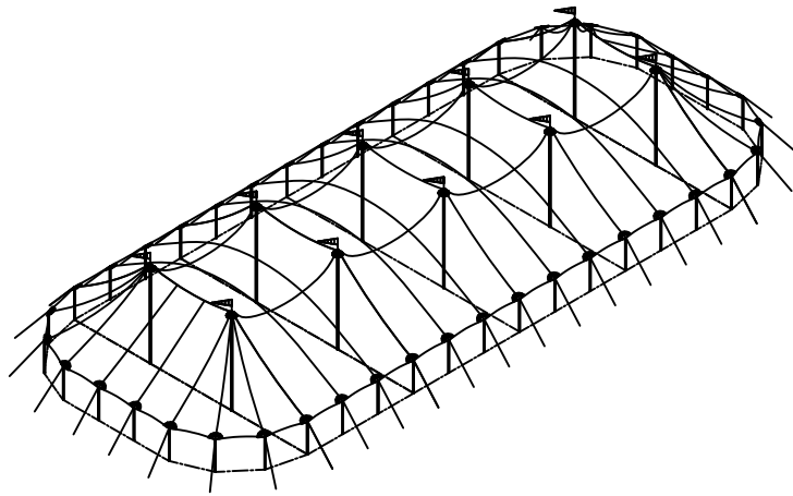
ISOMETRIC VIEW 10298 SQ. FT
