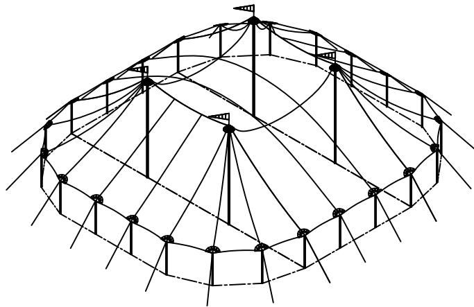
ISOMETRIC VIEW 4358 SQ. FT
