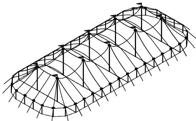
ISOMETRIC VIEW 10298 SQ. FT
