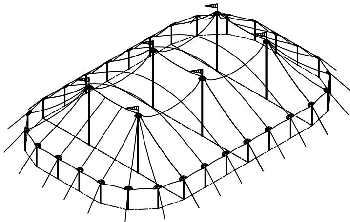
ISOMETRIC VIEW 6338 SQ. FT
