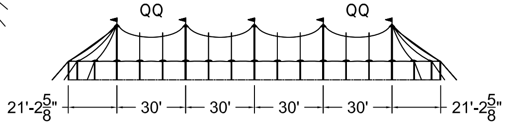
SIDE VIEW
