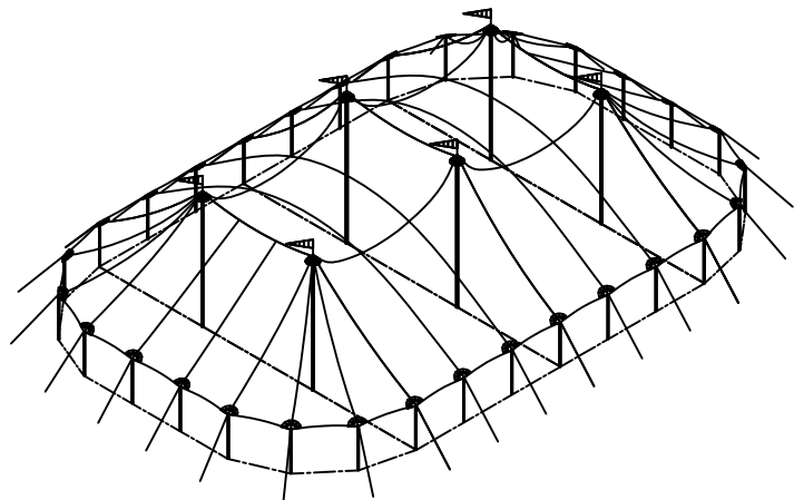
ISOMETRIC VIEW 6338 SQ. FT
