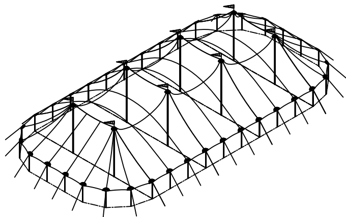
ISOMETRIC VIEW 8318 SQ. FT
