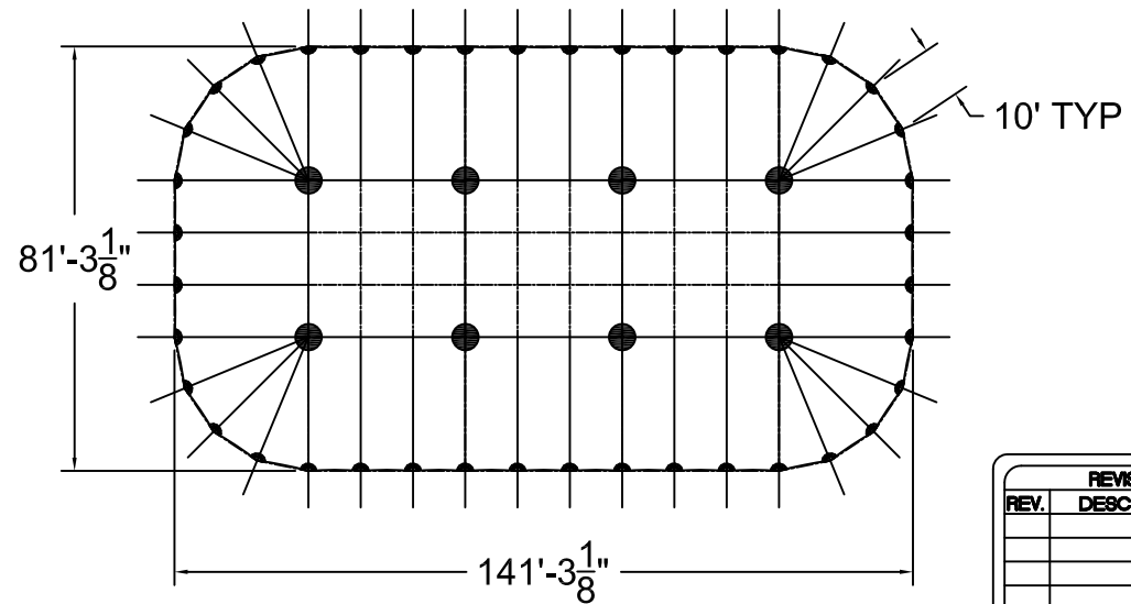
TOP VIEW
