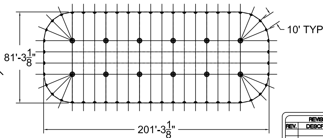
TOP VIEW
