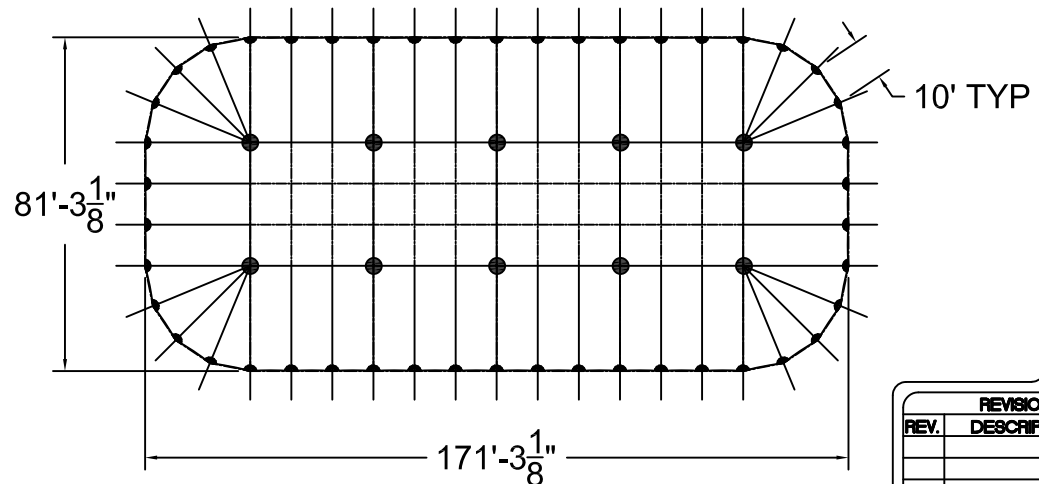
TOP VIEW
