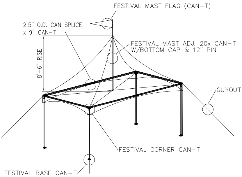
ISOMETRIC VIEW
