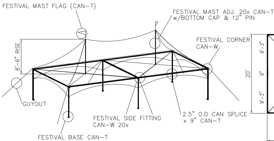
ISOMETRIC VIEW
