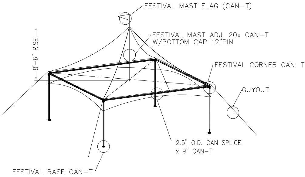
ISOMETRIC VIEW
