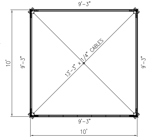
PLAN VIEW
