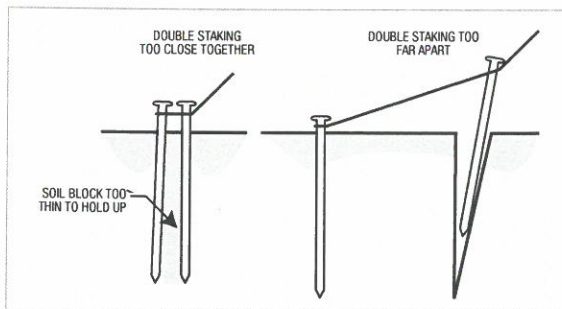
Figure 18. Double Staking Errors
