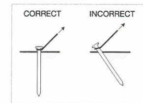
Figure 13. Stake Driving Angle
