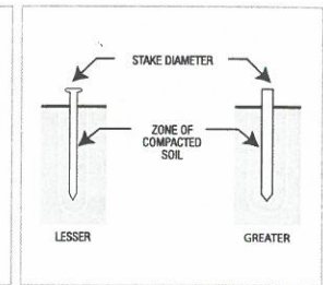
Figure 9. Stake Performance & Zone of Displaced Earth
