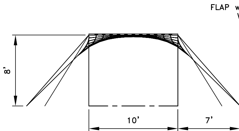
10' FRONT VIEW
