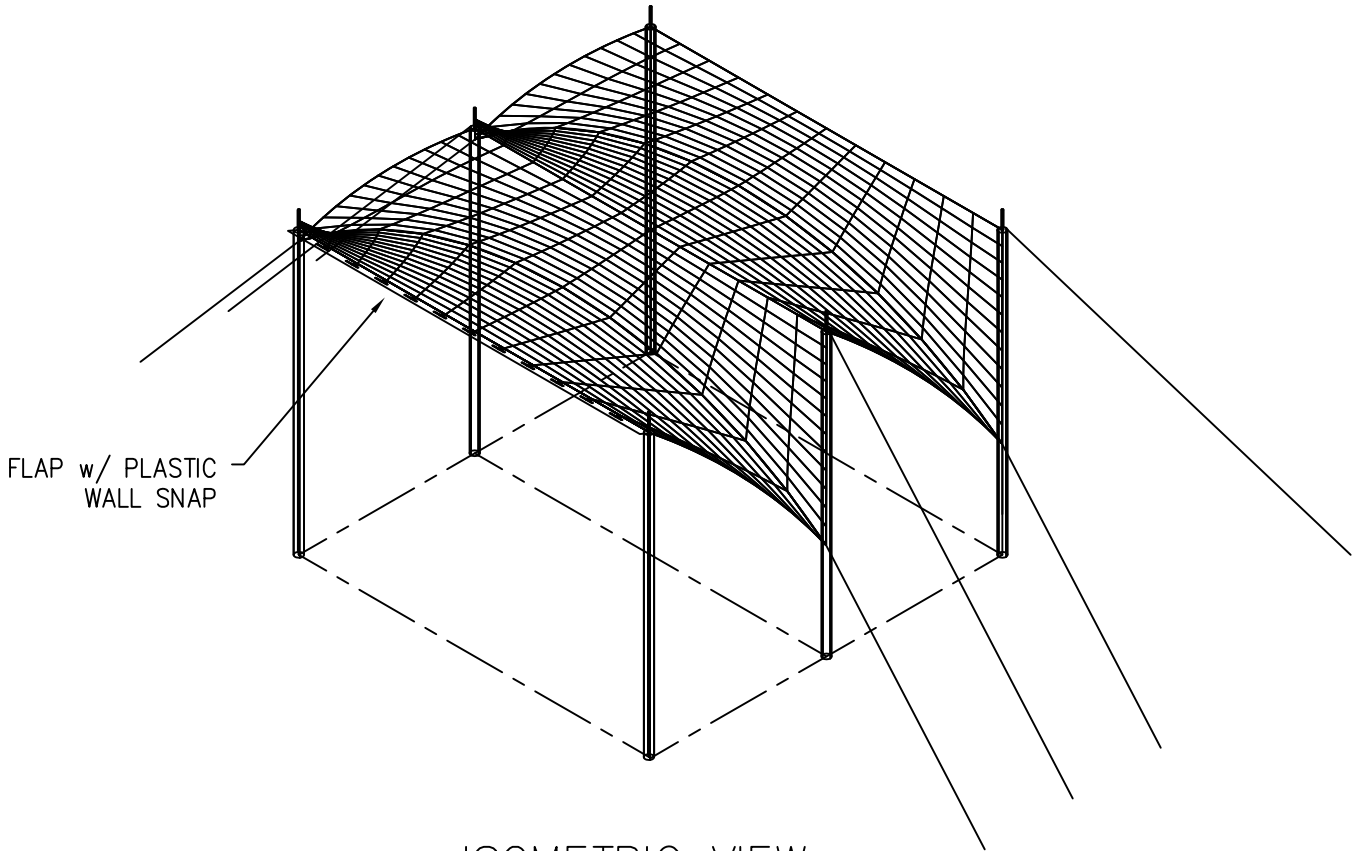
ISOMETRIC VIEW
