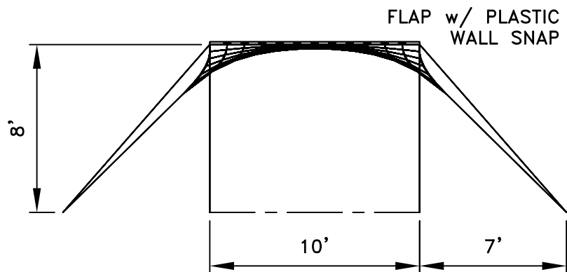
10' FRONT VIEW
