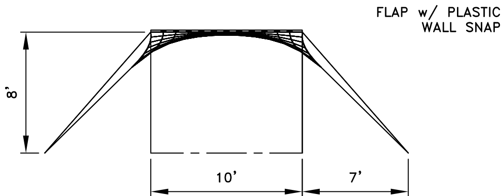
10' FRONT VIEW
