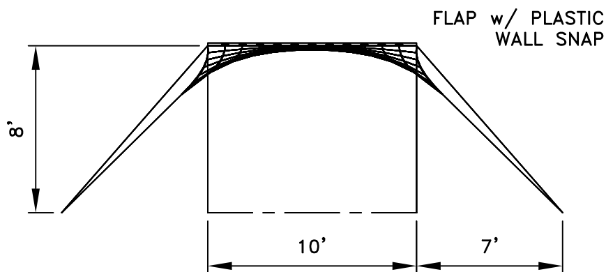
10' FRONT VIEW
