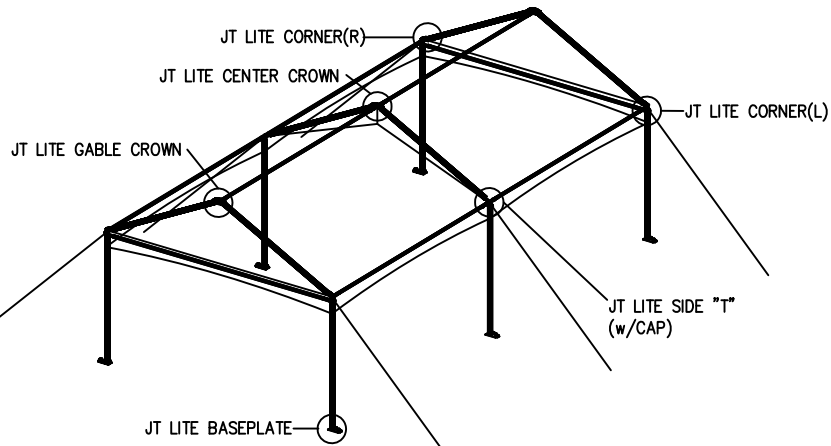
ISOMETRIC VIEW
