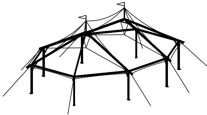
ISOMETRIC VIEW
