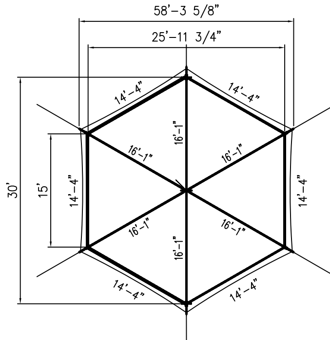
PLAN ELEVATION
