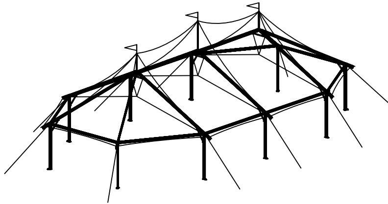
ISOMETRIC ELEVATION
