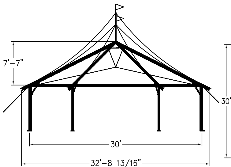
FRONT ELEVATION
