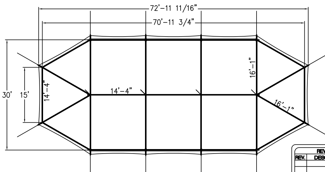
PLAN ELEVATION
