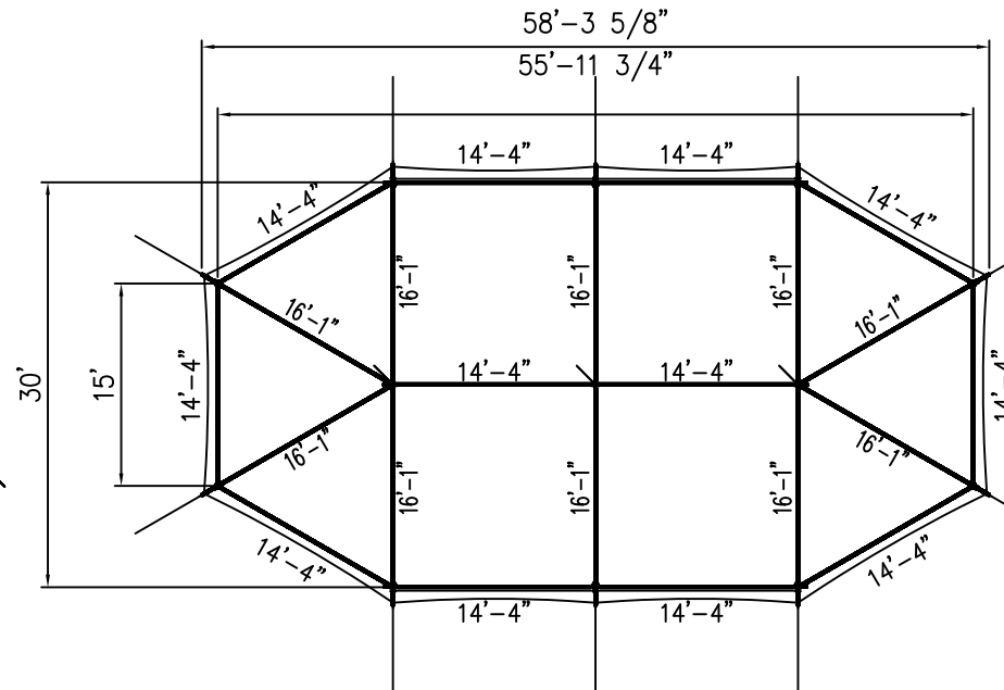
PLAN ELEVATION
