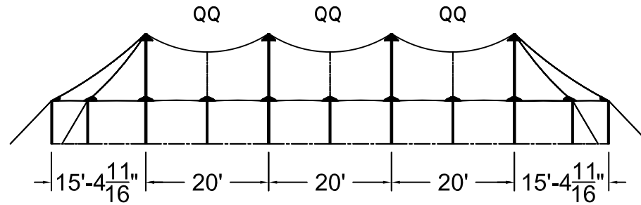
SIDE VIEW
