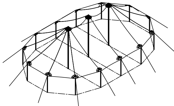
ISOMETRIC VIEW 1417 SQ. FT
