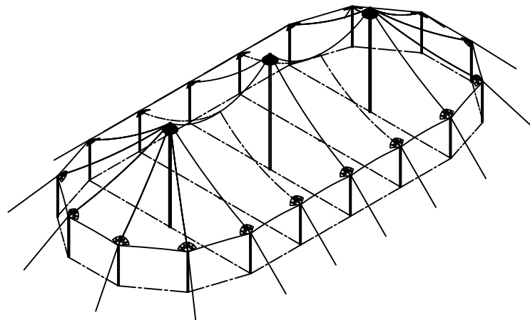
ISOMETRIC VIEW 2064 SQ. FT
