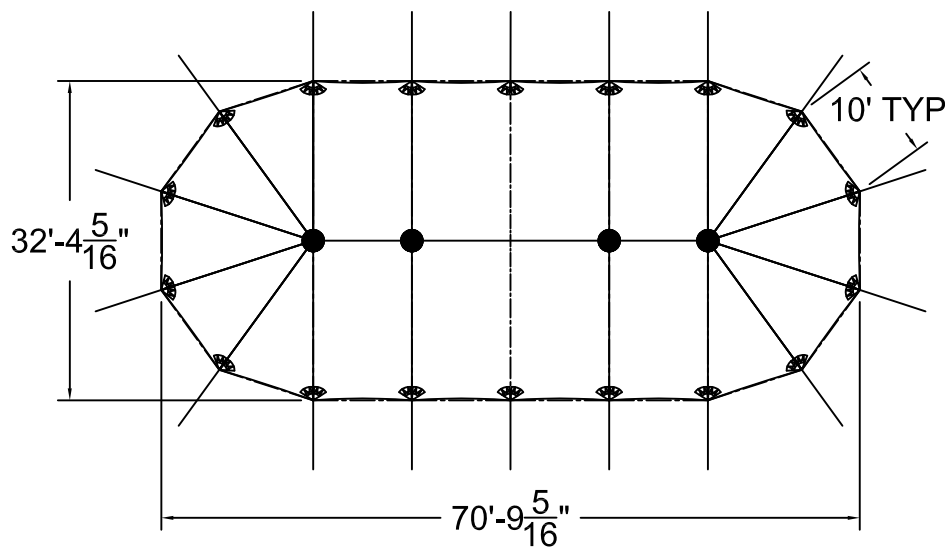
TOP VIEW
