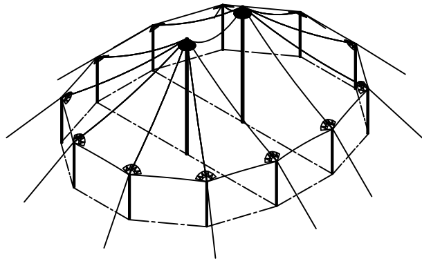
ISOMETRIC VIEW 1093 SQ. FT
