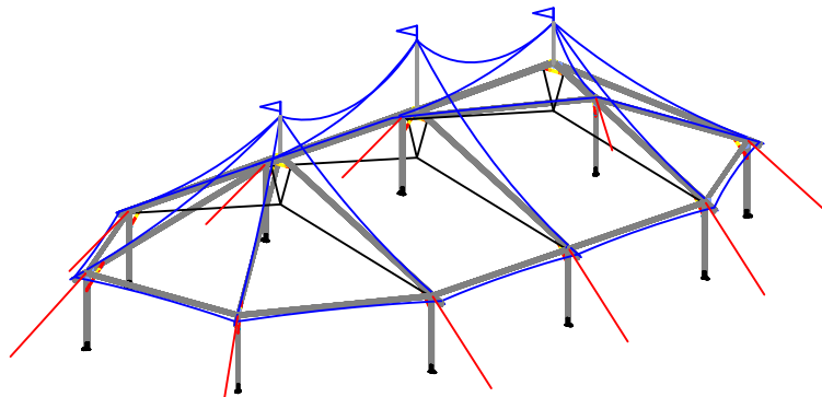
ISOMETRIC ELEVATION
