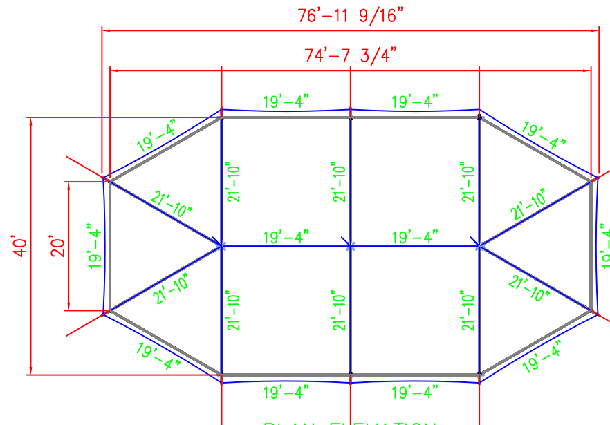
PLAN ELEVATION
