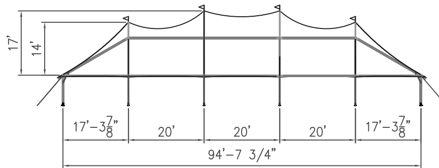
SIDE ELEVATION
