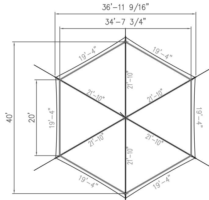
PLAN ELEVATION
