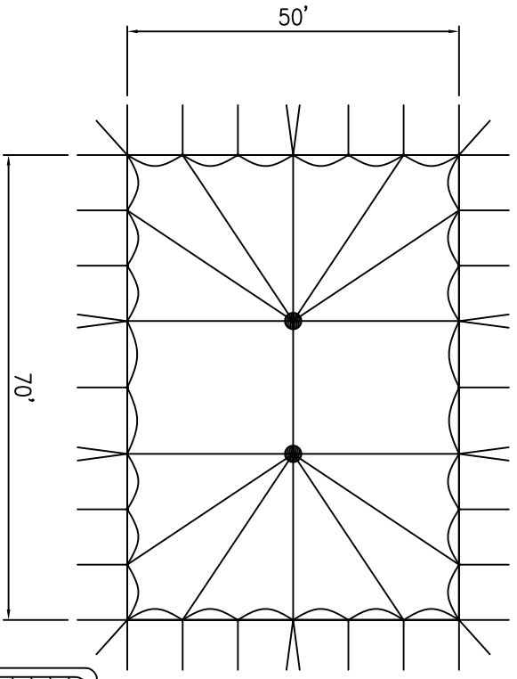
PLAN VIEW
