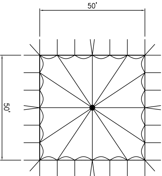
PLAN VIEW
