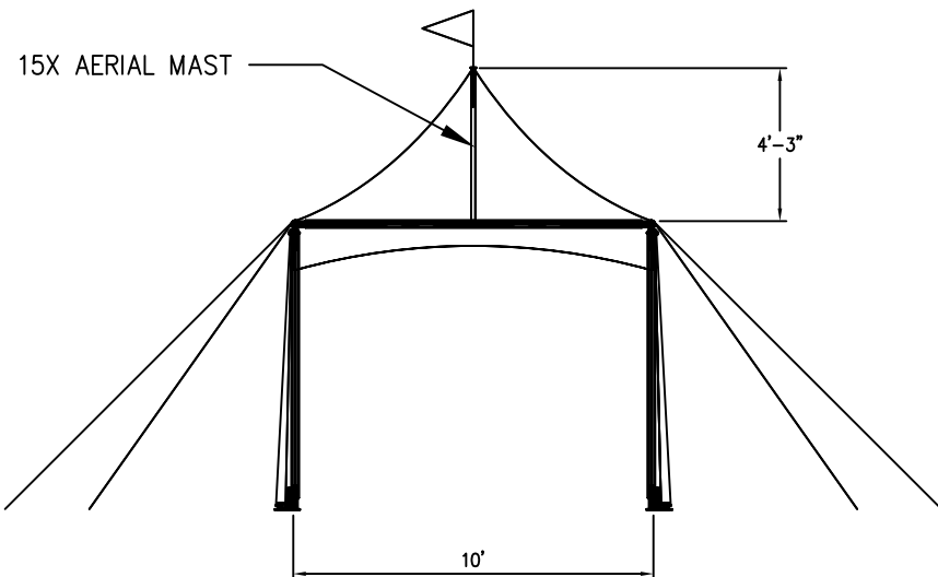
END VIEW
