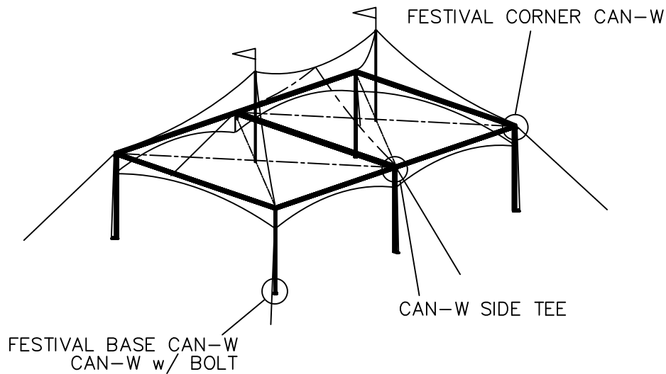
ISOMETRIC VIEW
