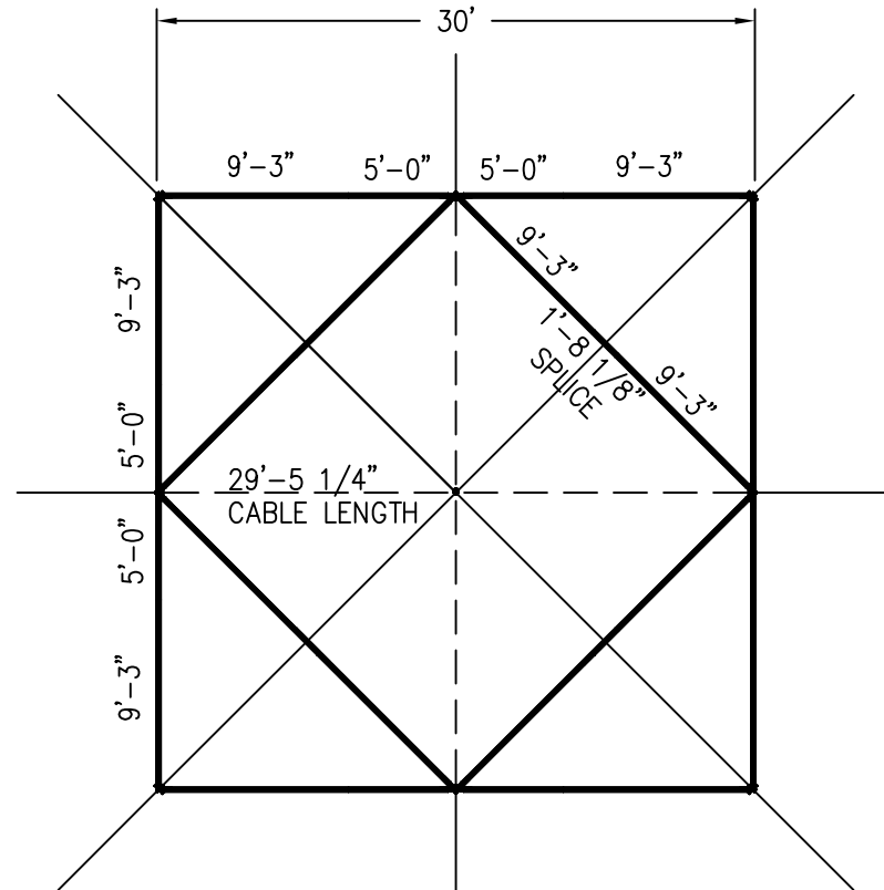
PLAN VIEW
