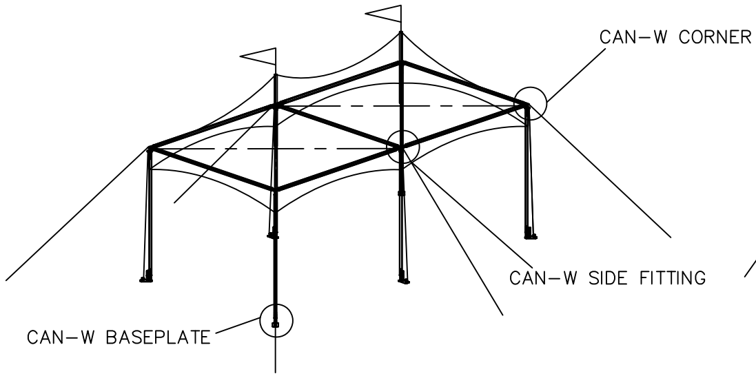
ISOMETRIC VIEW
