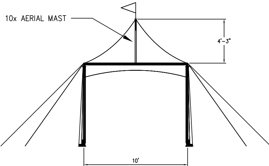
END VIEW
